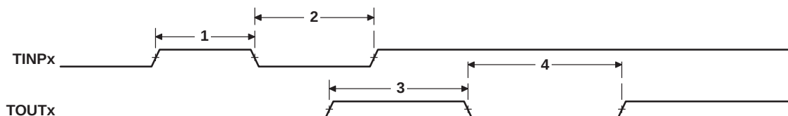
Figure 57. Timer Timing
