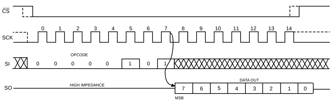
Figure 5. RDSR Timing
