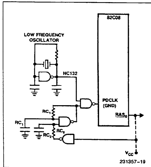
Figure 9. Low Frequency Oscillator
