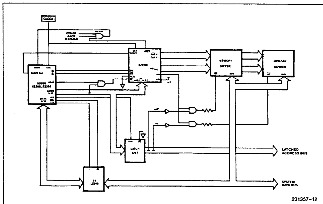
Figure 3B. 82C08 interface to an 80286
