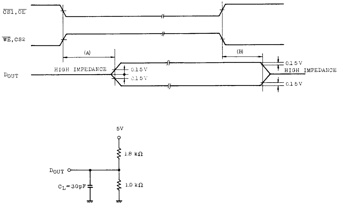
Fig.1 Output load condition for enable disable time measurement.
