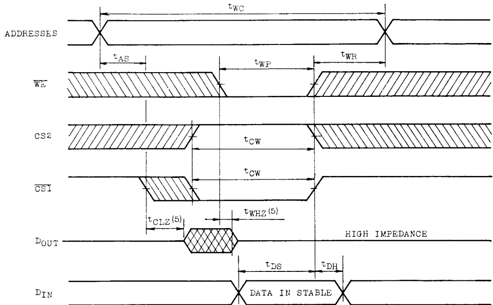
WRITE CYCLE 2 (4) ( \overline{\text{CS1}} Controlled Write)
