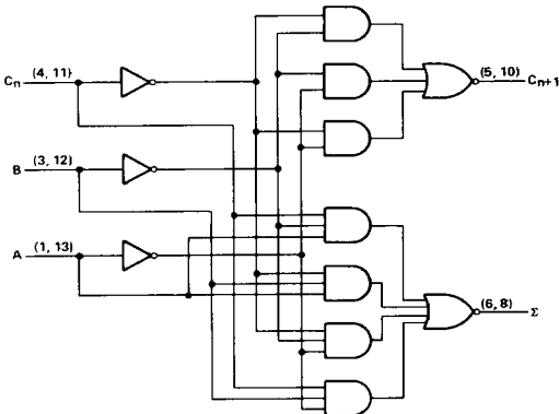
logic diagram (each adder)
