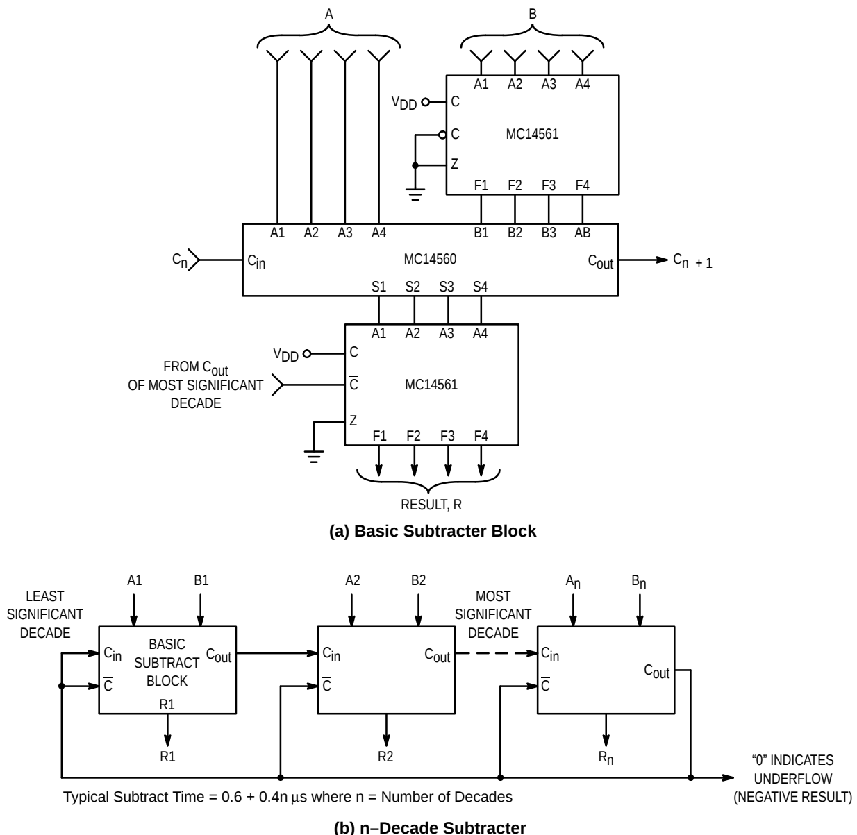
Figure 6. Subtraction of Unsigned NBCD Numbers
