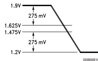
FIGURE 9. Noise Margin
