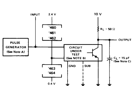
TEST CIRCUIT
