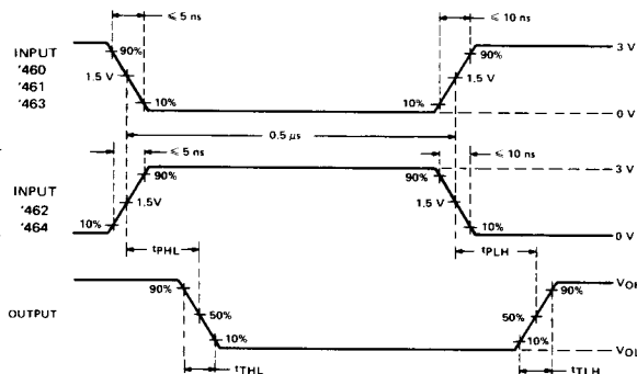
VOLTAGE WAVEFORMS
