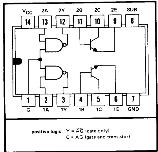
SN55460 ... J SN75460 ... J OR N DUAL-IN-LINE PACKAGE (TOP VIEW)
