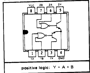
SN55463 ... JG SN75463 ... JG OR P DUAL-IN-LINE PACKAGE (TOP VIEW)
