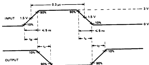
VOLTAGE WAVEFORMS
