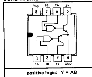
SN55461 ... JG SN75461 ... JG OR P DUAL-IN-LINE PACKAGE (TOP VIEW)
