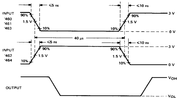
VOLTAGE WAVEFORMS
