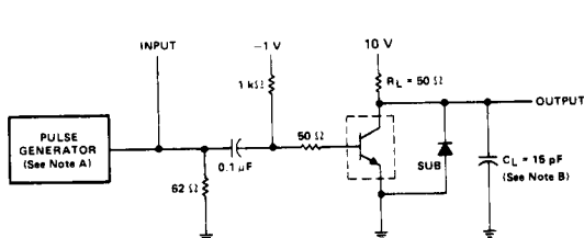
TEST CIRCUIT
