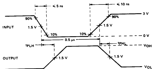
VOLTAGE WAVEFORMS
