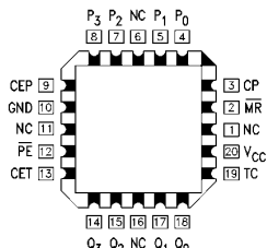
Pin Assignment for LCC 'F161A
