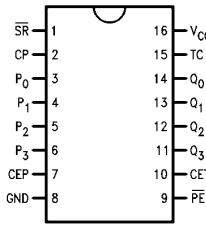
Pin Assignment for DIP, SOIC and Flatpak 'F163A
