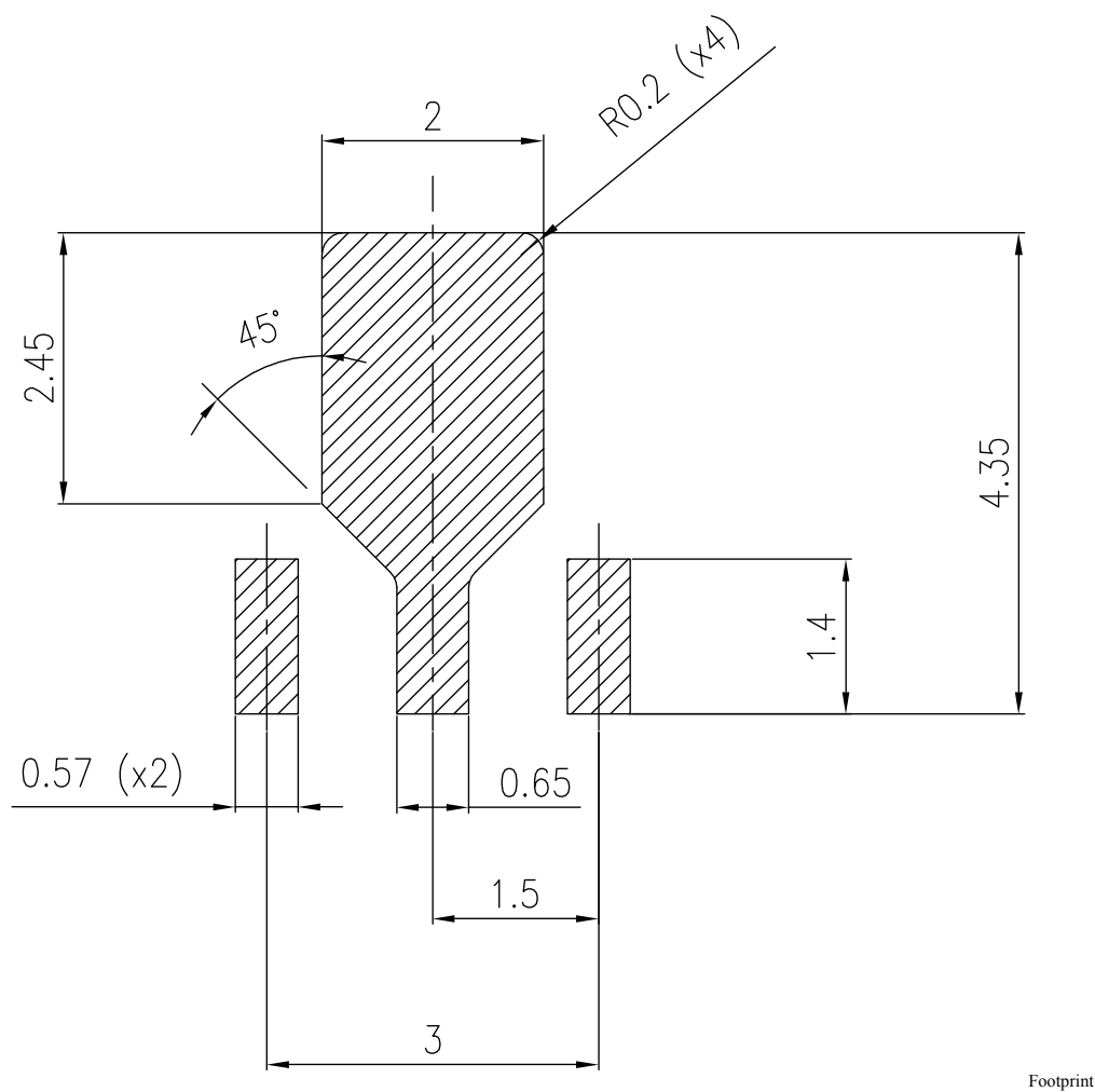
Figure 25. SOT-89 recommended footprint
