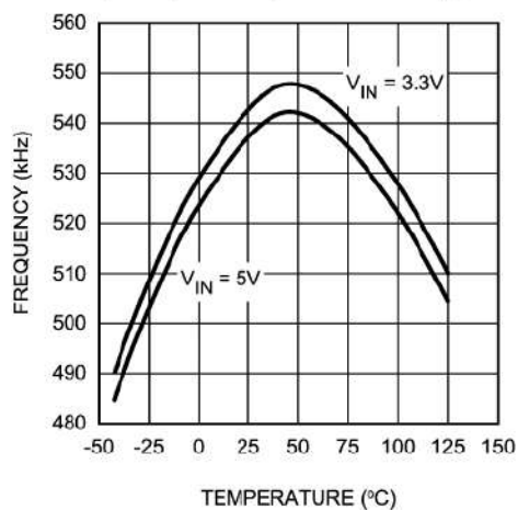
Frequency vs Temperature and V_{IN}
