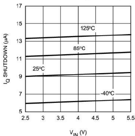
Shut-Down Current vs V_{IN} and Temp.
