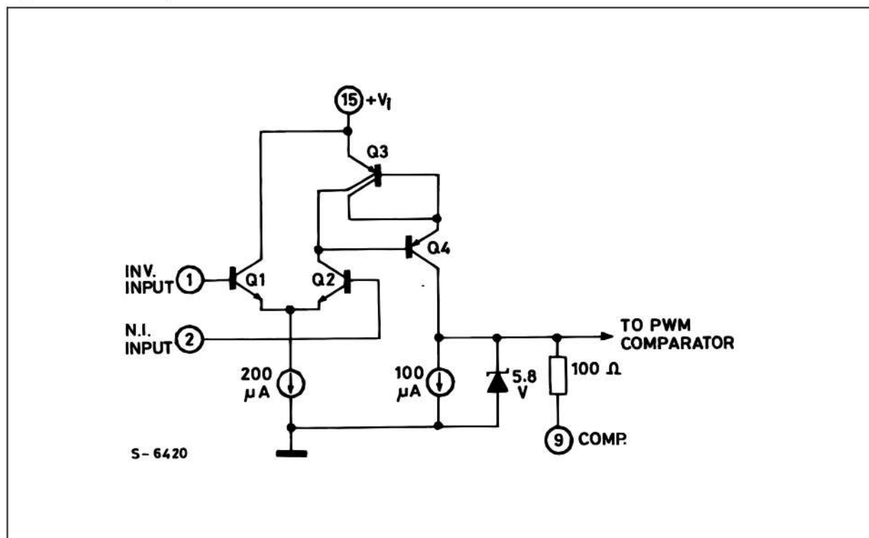
Figure 5 : Error Amplifier.
