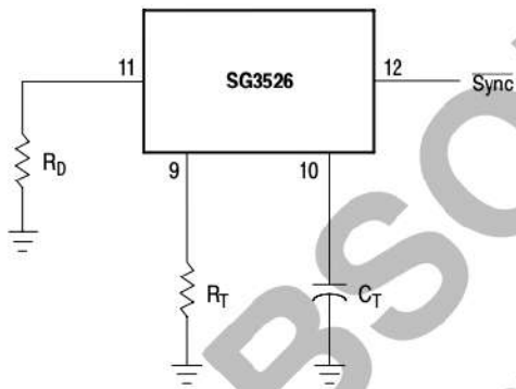
Figure 15. Oscillator Connections
