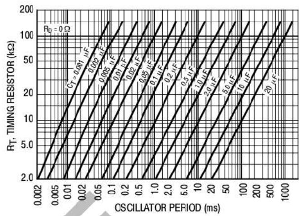
Figure 9. Oscillator Period
