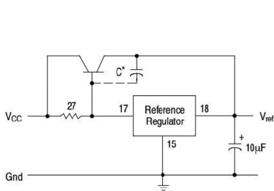
Figure 13. Extending Reference Output Current Capability
