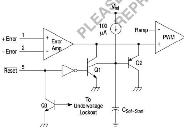
Figure 17. Soft-Start Circuitry
