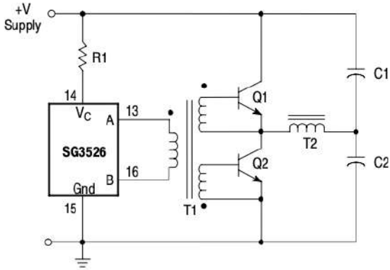
Figure 19. Half-Bridge Configuration
