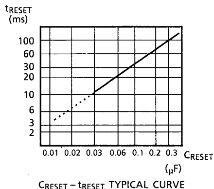
C RESET – t RESET TYPICAL CURVE
