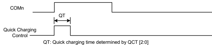
R Type Bias Configuration – 1/3 Bias
