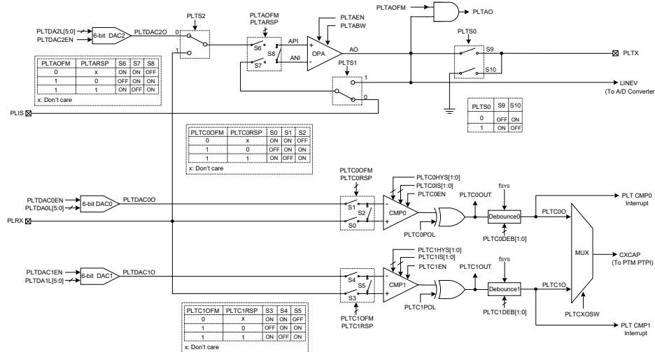
Power Line Data Transceiver Block Diagram
