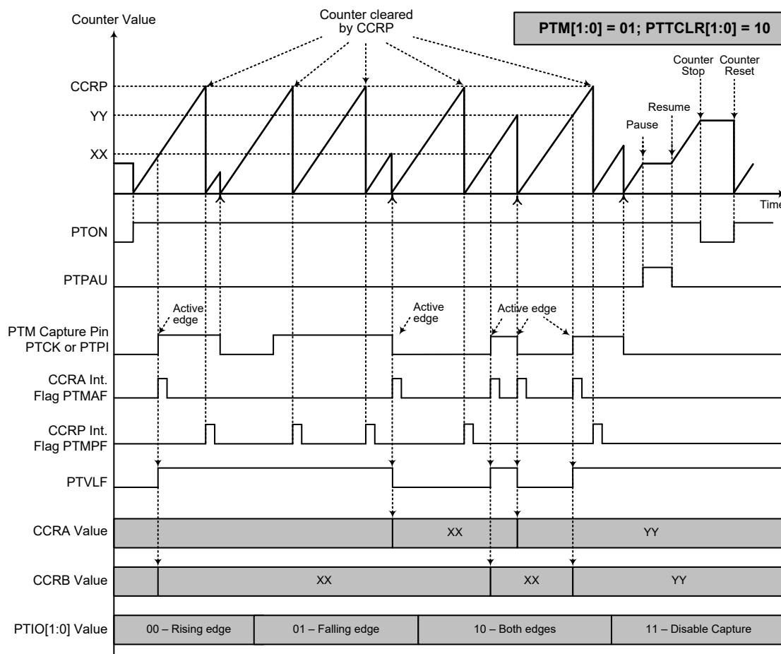
Capture Input Mode – PTTCLR[1:0]=10
