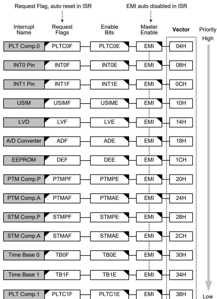
Interrupt Structure
