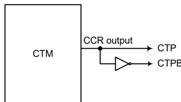
CTM Function Pin Block Diagram
