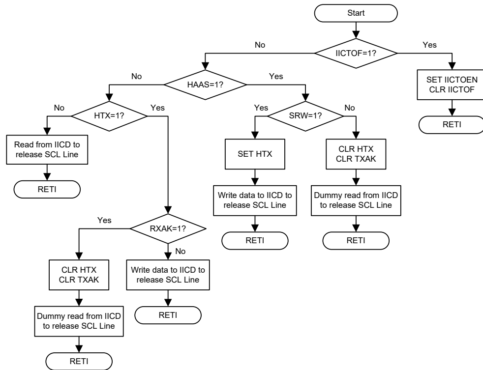
I²C Bus ISR Flowchart
