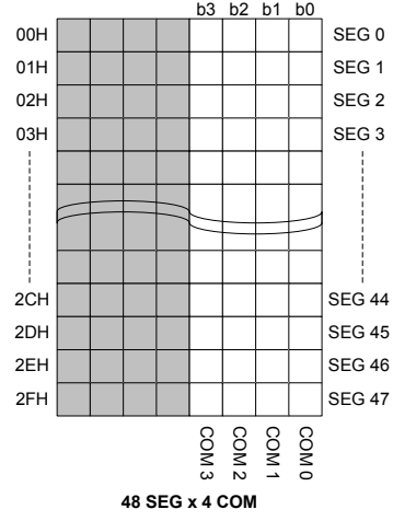
BS67F370 LCD Memory Map
