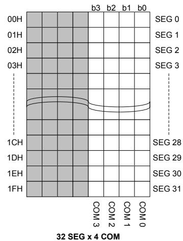
BS67F350 LCD Memory Map
