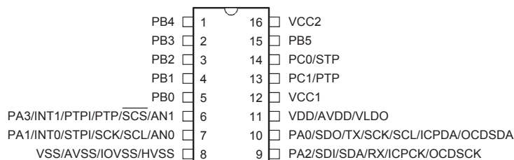
HT66F2730/HT66V2730 16 NSOP-EP-A
