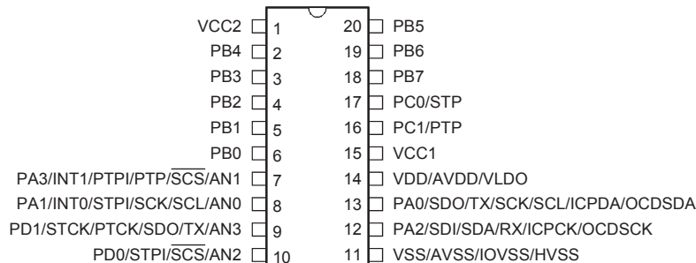
HT66F2730/HT66V2730 20 NSOP-A
