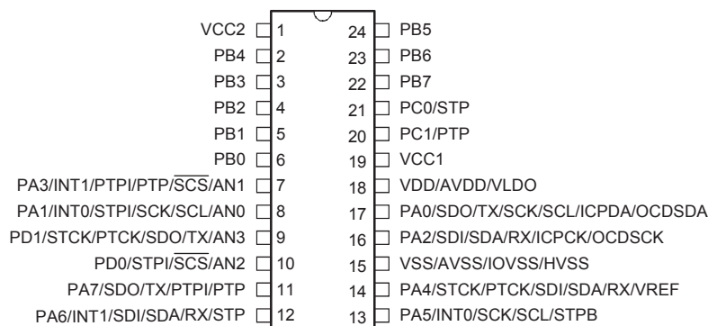
HT66F2730/HT66V2730 24 SOP-A/SSOP-EP-A
