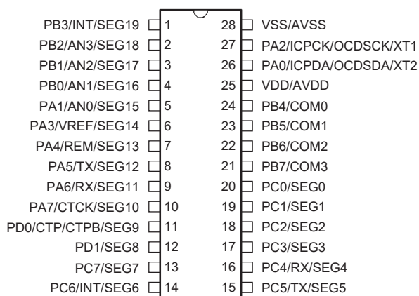
HT67F2432/HT67V2432 28 SOP-A/SSOP-A
