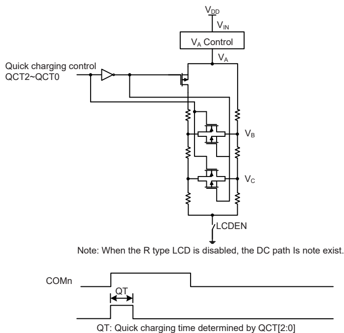
R Type Bias Voltage Configuration – 1/3 Bias (n=0~3)
