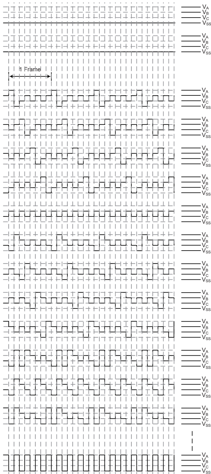
LCD Driver Output – Type A, 1/4 Duty, 1/3 Bias
