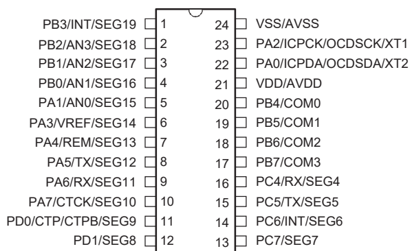
HT67F2432/HT67V2432 24 SOP-A/SSOP-A
