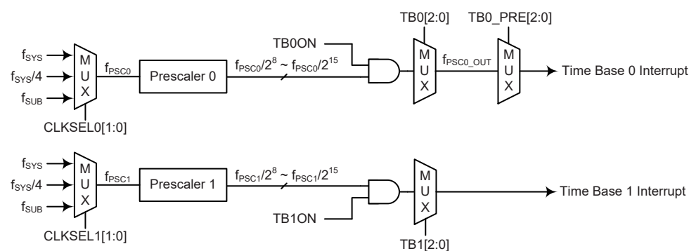
Time Base Interrupts
