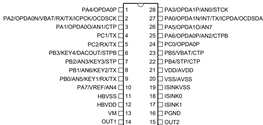
BS45F3345/BS45V3345 28 SSOP-A
