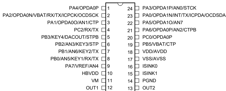
BS45F3345/BS45V3345 24 SSOP-A
