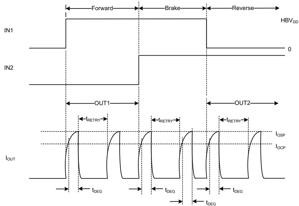
Retry Mechanism
