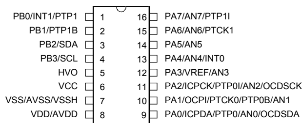
HT45F3630/HT45V3630 16 SSOP-A
