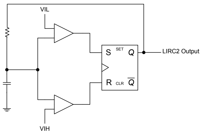
LIRC2 Oscillator
