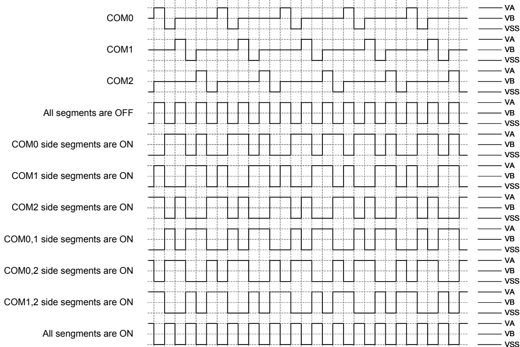
LCD Driver Output – Type A, 1/3 Duty, 1/2 Bias
