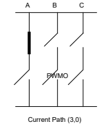
Mask Independent Mode Example
