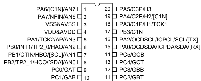
HT66FM5240 20 SSOP-A
