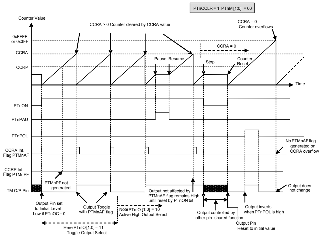
Compare Match Output Mode – PTnCCLR=1
