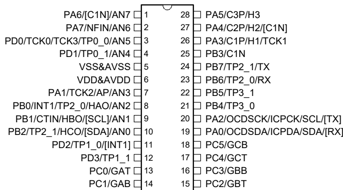
HT66FM5240 28 SSOP-A
