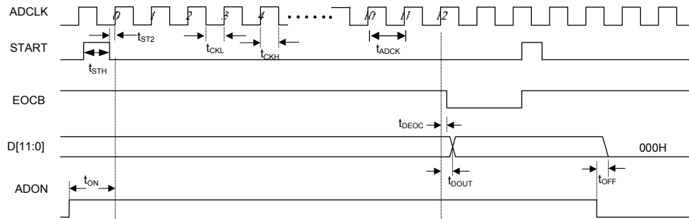
A/D Conversion Timing Diagram
