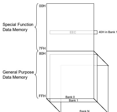
Data Memory Sturcture
