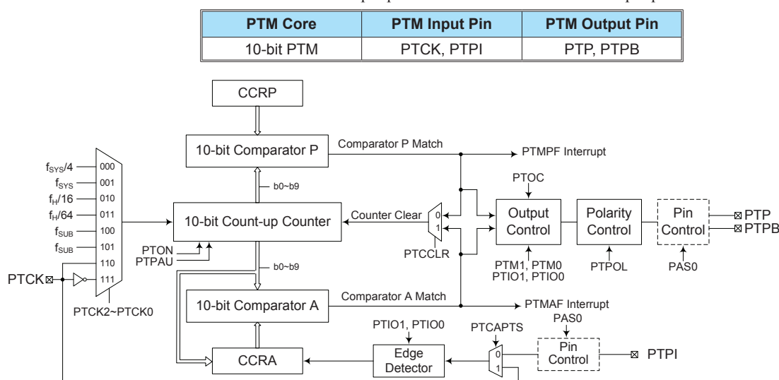
Periodic Type TM Block Diagram
