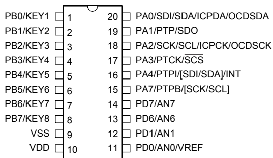
BS84B08C/BS84BV08C 20 NSOP-A/SOP-A/SSOP-A
