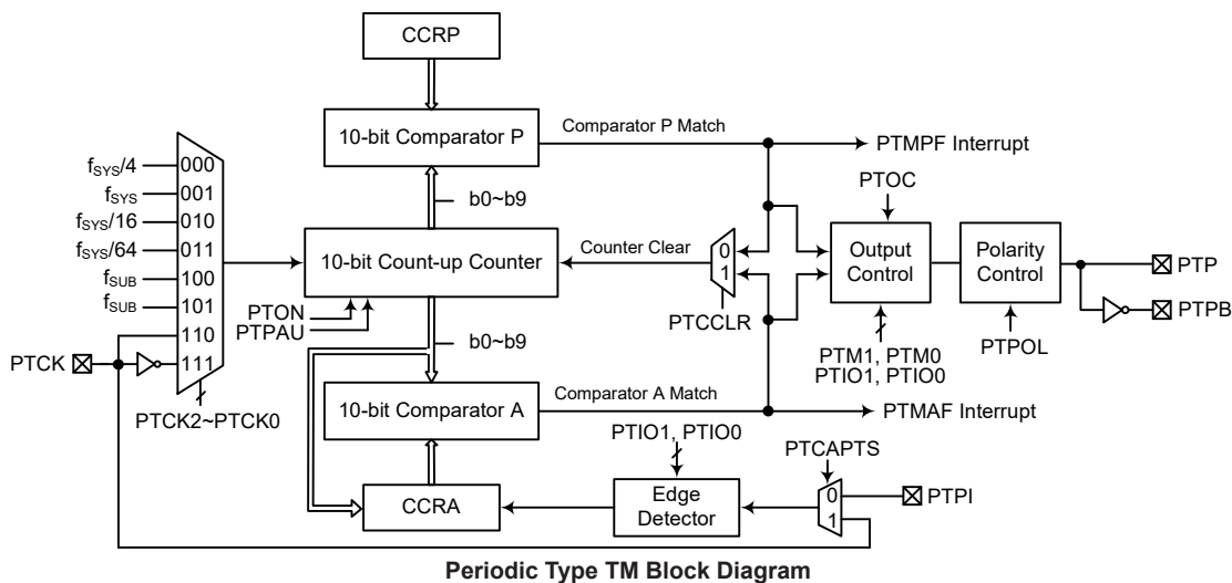
Periodic Type TM Block Diagram
