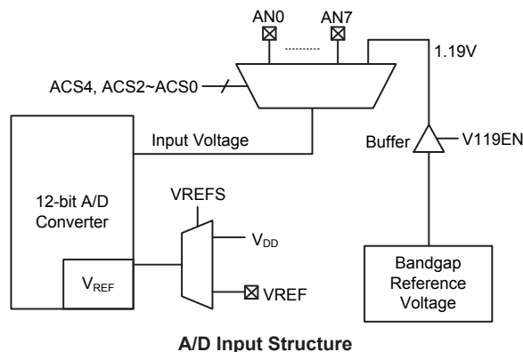
A/D Input Structure
