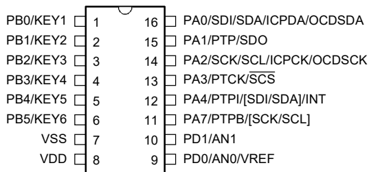
BS84B08C/BS84BV08C 16 NSOP-A/SSOP-A
