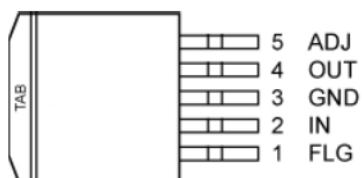
5-Pin TO-263 (D'Pak) Adjustable with Flag (U) MIC29153/29303/29503
