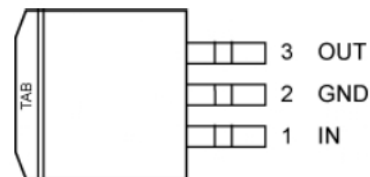
3-Pin TO-263 (D'Pak) (UT) MIC29150/29300
