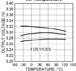
MIC29750-3.3 Output Voltage vs. Temperature
