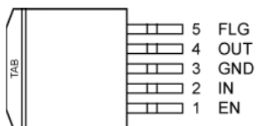
5-Pin TO-263 (D'Pak) Fixed Voltage (U) MIC29151/29301/29501
