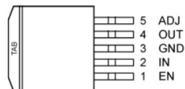
5-Pin TO-263 (D'Pak) Adjustable Voltage (U) MIC29302/29502
