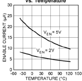
MIC29501-xx/2 Enable Current vs. Temperature
