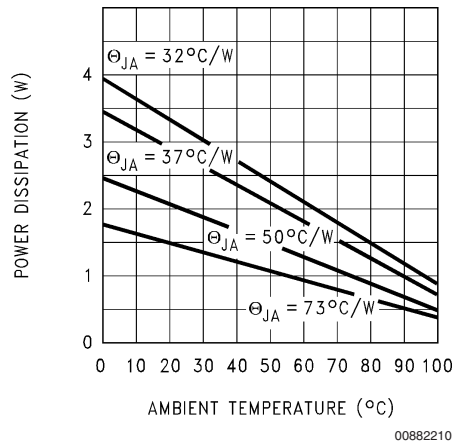
Maximum Power Dissipation (TO-263) See (Note 2)
