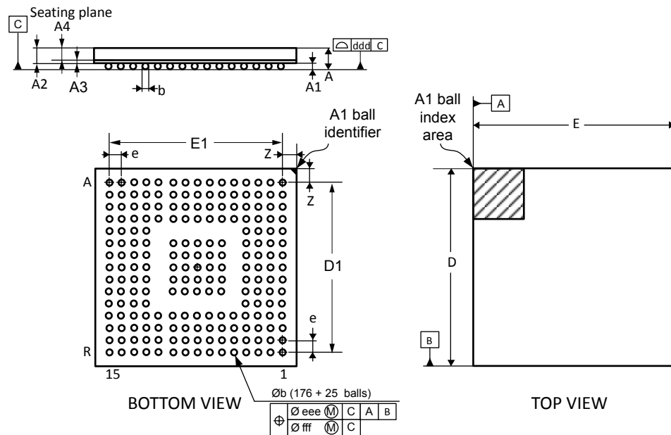
Figure 88. UFBGA176+25 - Outline
