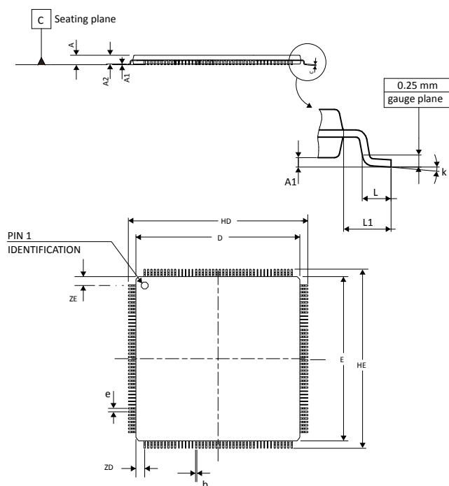
Figure 82. LQFP176 - Outline
