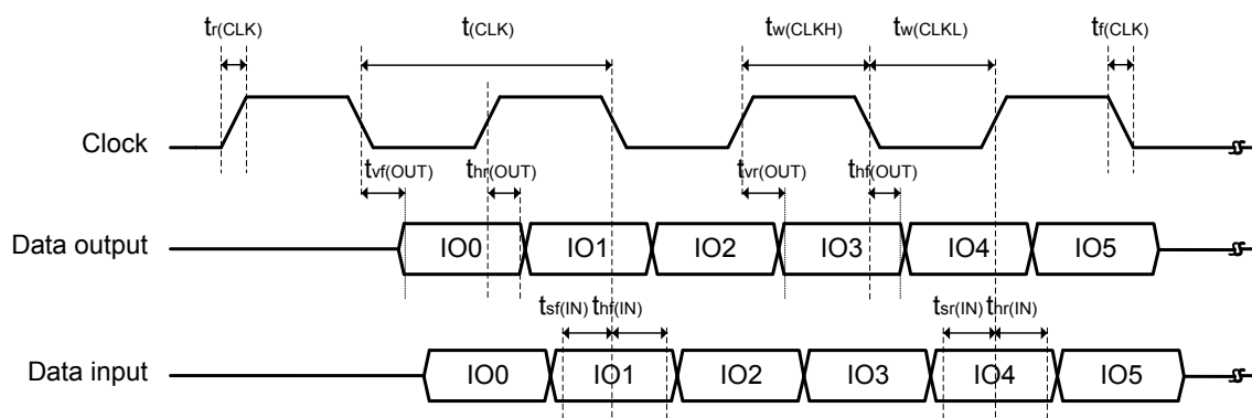
Figure 69. DDR mode
