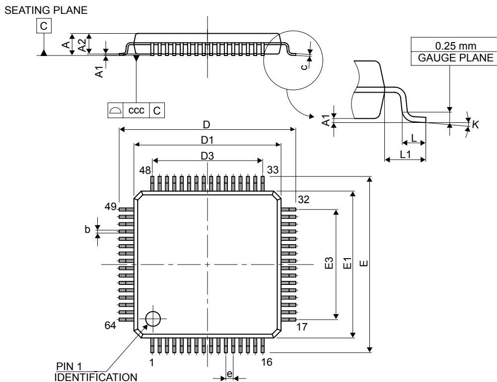
Figure 73. LQFP64 - Outline
