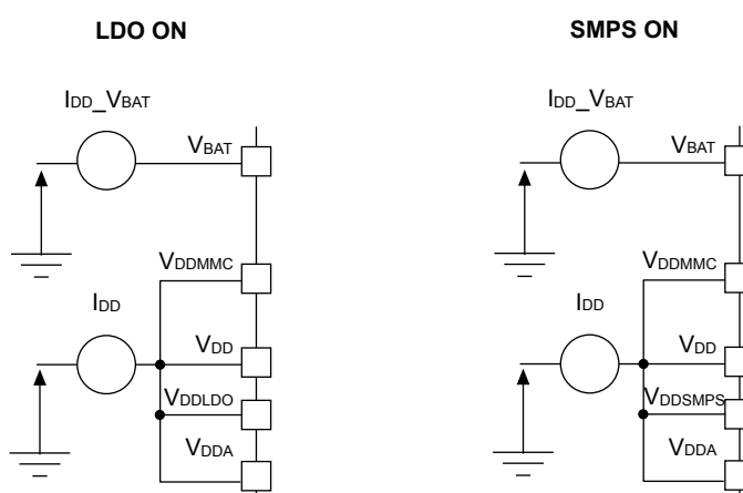
Figure 13. Current consumption measurement scheme
