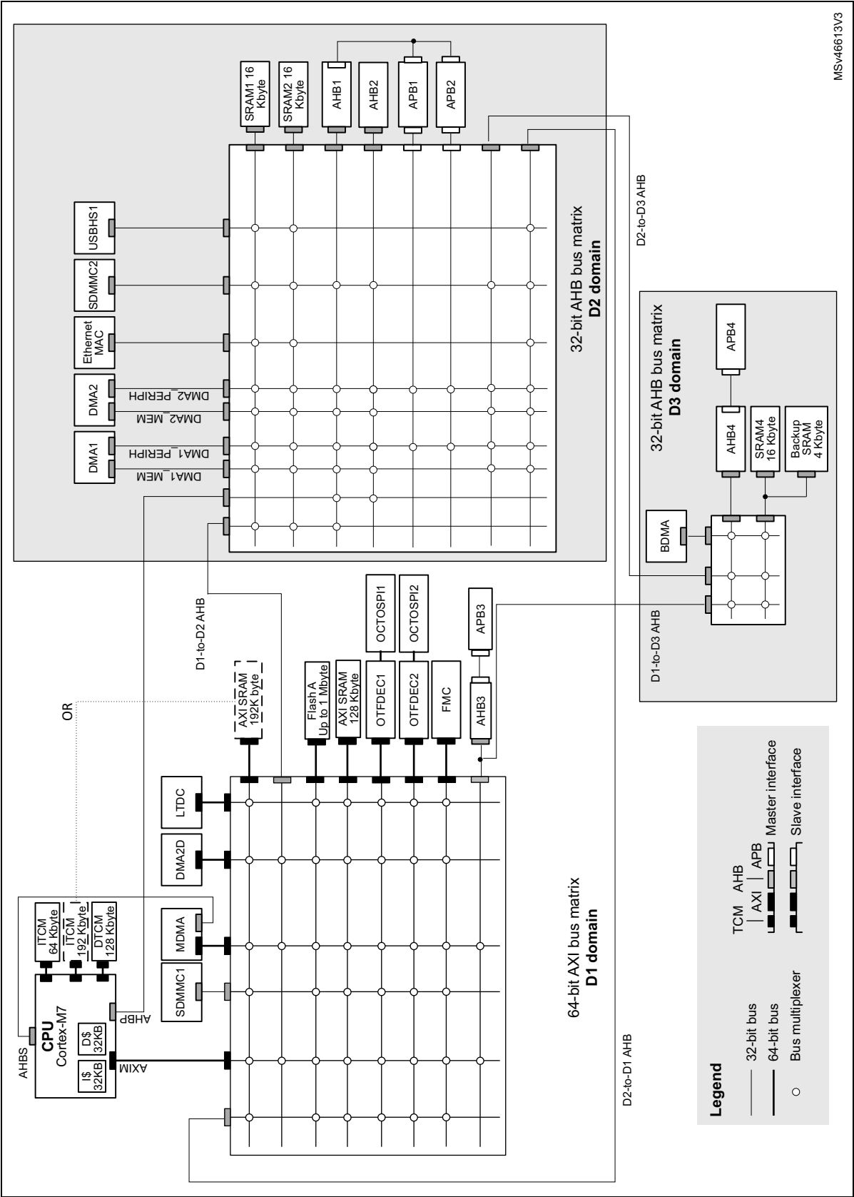
Figure 3. STM32H735xG bus matrix
