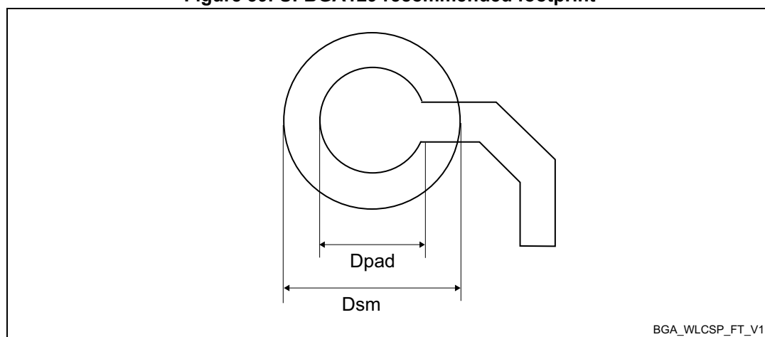
Figure 39. UFBGA129 recommended footprint
