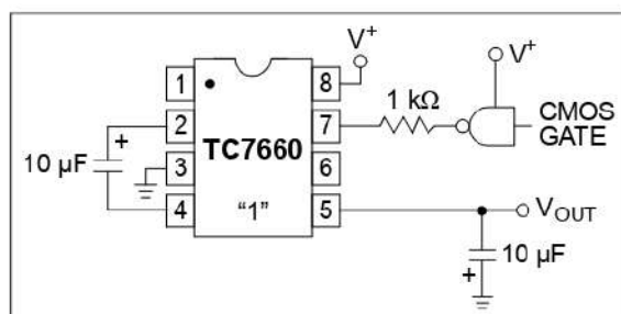
FIGURE 5-4: External Clocking.
