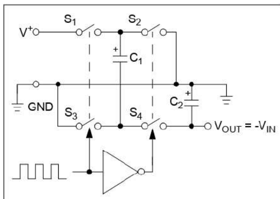
FIGURE 4-1: Ideal Switched Capacitor Inverter.
