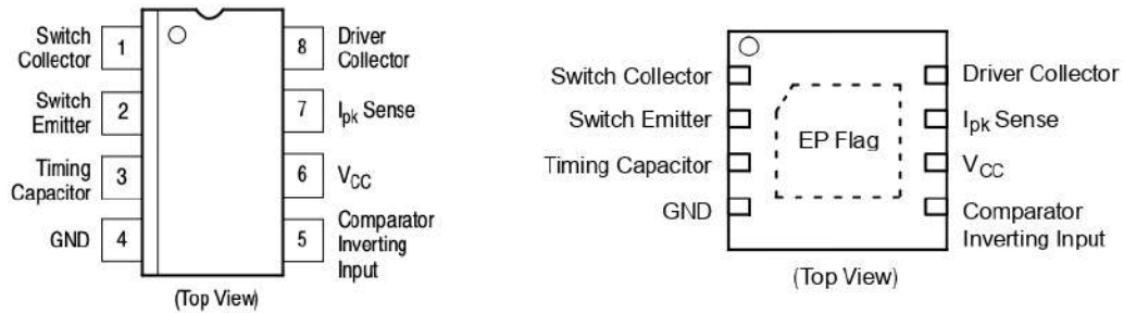
Figure 2. Pin Connections
