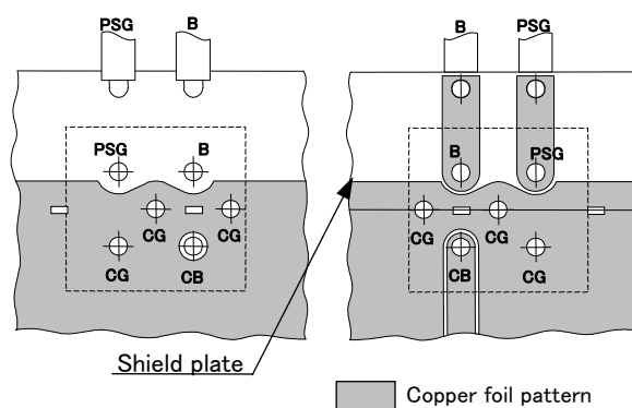
(1) COMPONENT SIDE VIEW (2) BOTTOM VIEW
