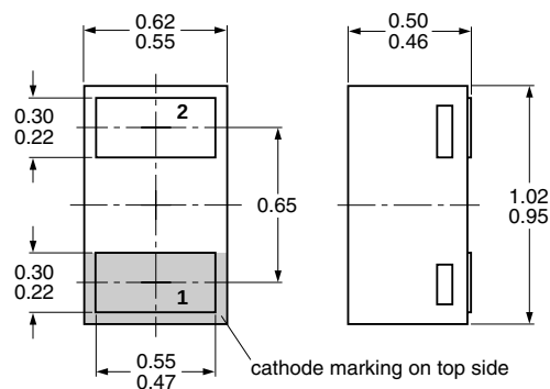
Fig 9. Package outline SOD882
