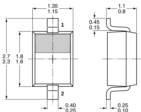
Fig 5. Package outline SOD323 (SC-76)
