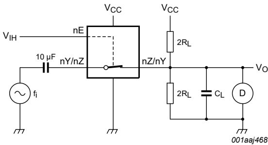
Fig. 14. Test circuit for measuring total harmonic distortion
