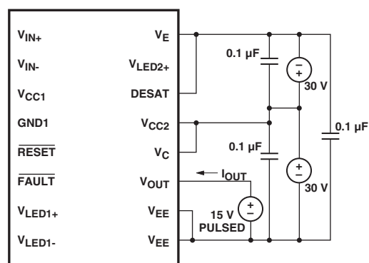
Figure 33. I_{\text{OL}} pulsed test circuit.
