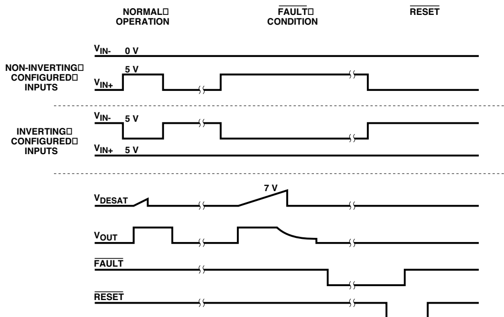
Figure 63. Timing diagram.
