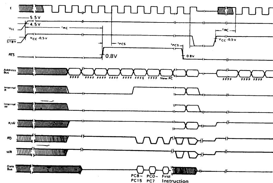
Figure 11 Reset Timing
