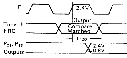
(a) Timer 1 Output Timing
