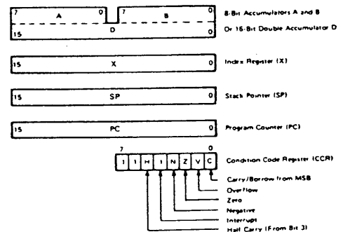
Figure 23 CPU Programming Model
