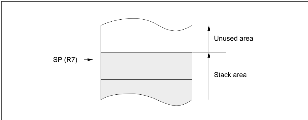
Figure 2-2 Stack Pointer
