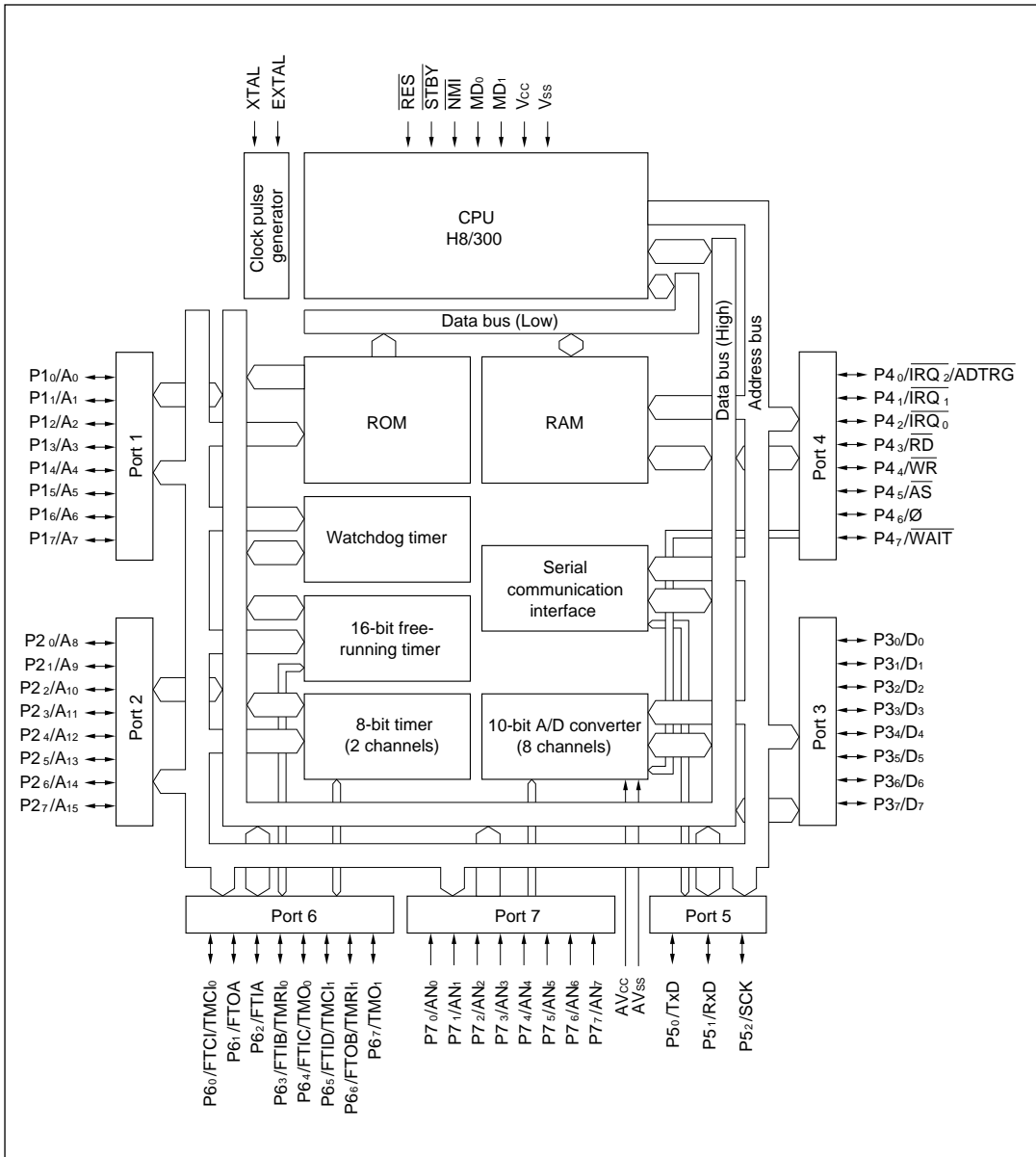
Figure 1-1 Block Diagram
