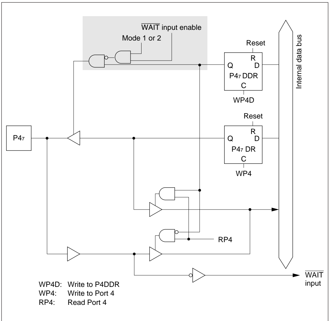
Figure C-4 (e) Port 4 Block Diagram (Pin P47)
