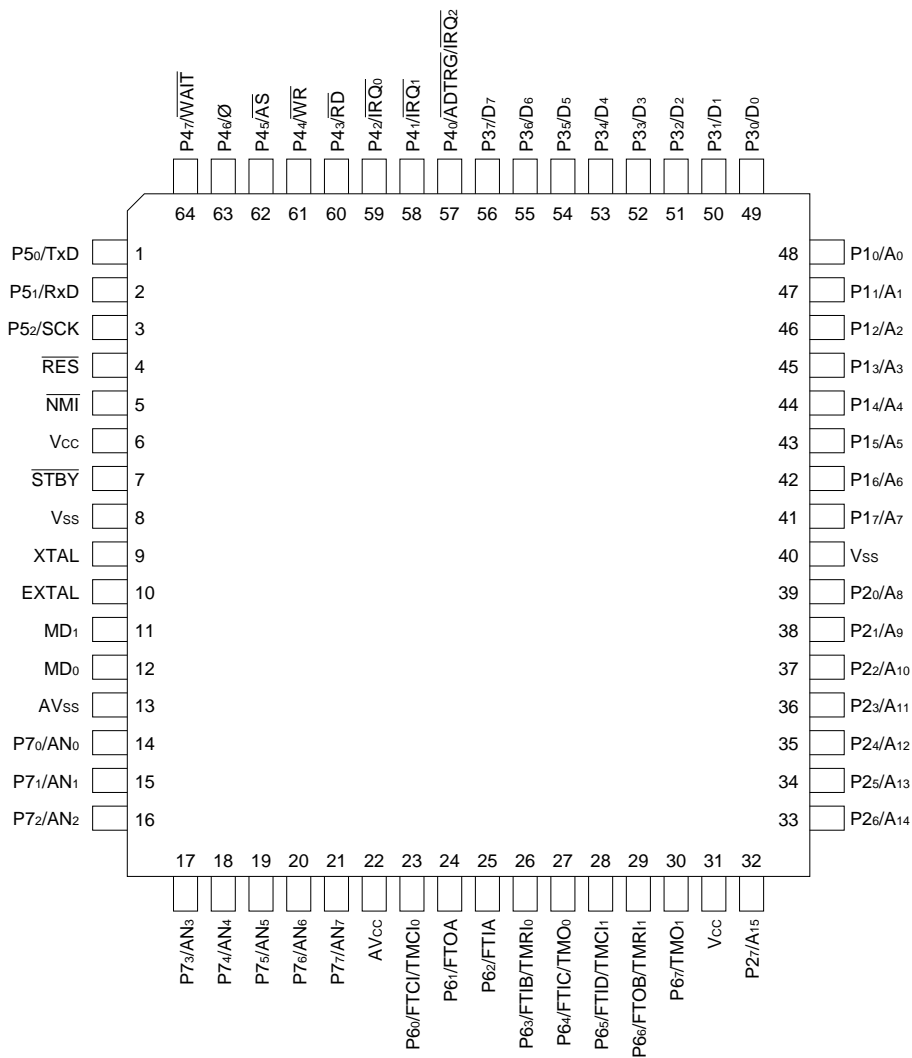
Figure 1-3 Pin Arrangement (FP-64A, Top view)
