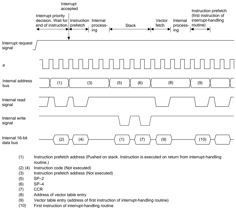
Figure 4-6 Timing of Interrupt Sequence
