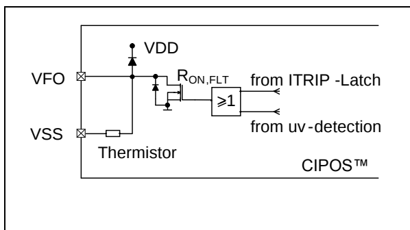
Figure 5: Internal circuit at pin VFO
