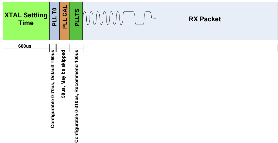
Figure 9. RX Timing
