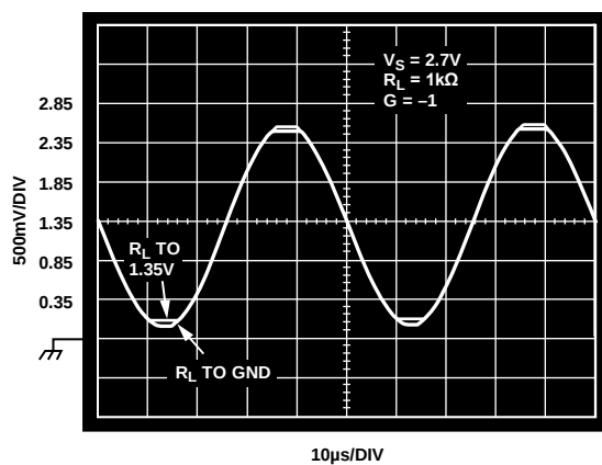
Figure 40. Output Swing
