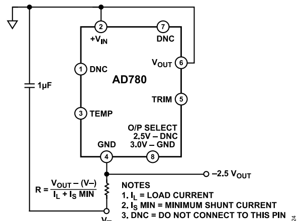
Figure 24. Negative (–2.5 V Shunt Mode Reference)
