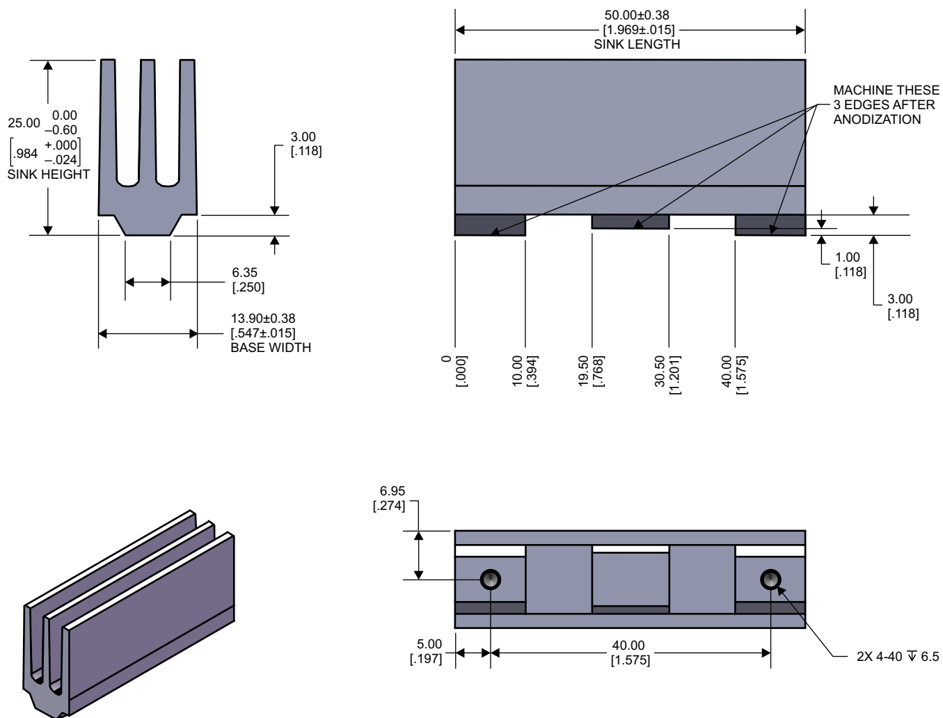
Figure 24. EVM Heatsink
