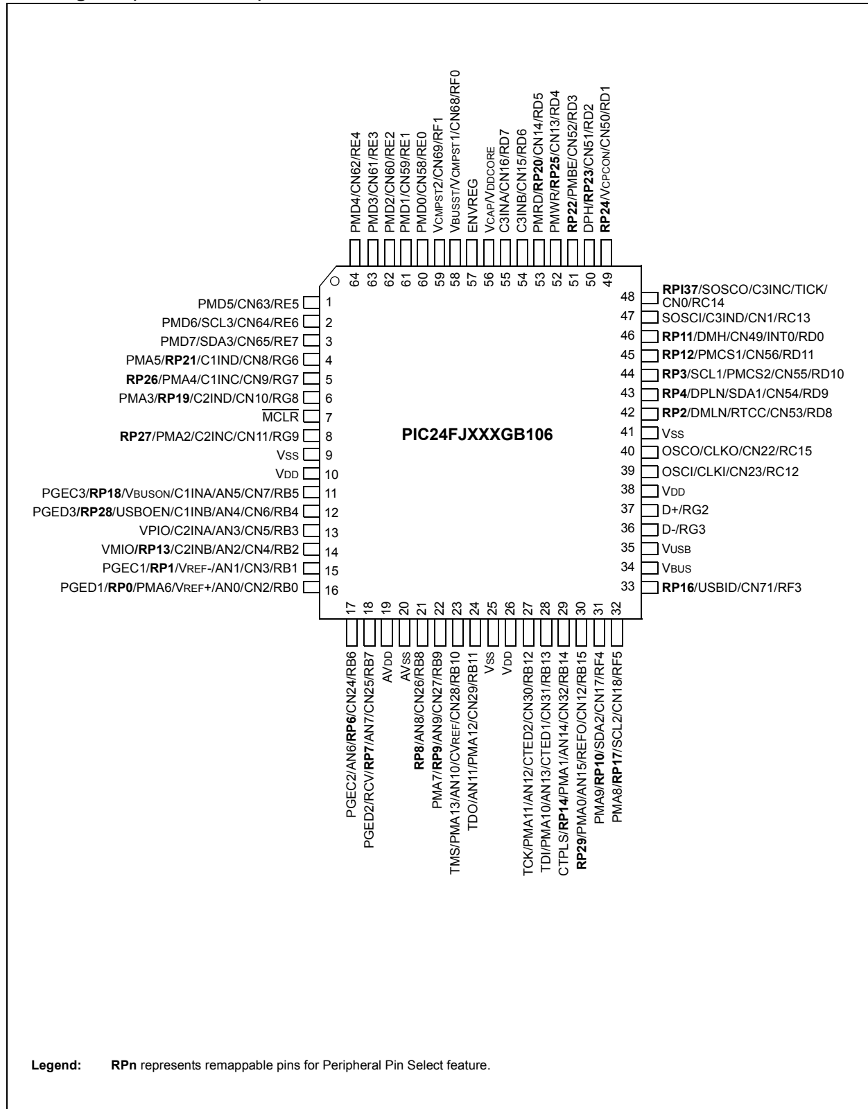
Pin Diagram (64-Pin TQFP)
