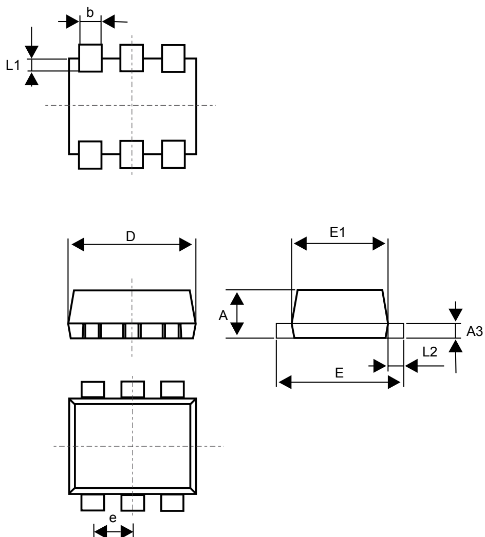
Figure 20. SOT-666 package outline
