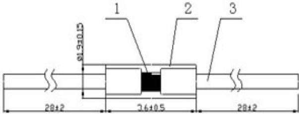
MF58Z •1---chip, 2---glass encapsulation, 3---lead wire
